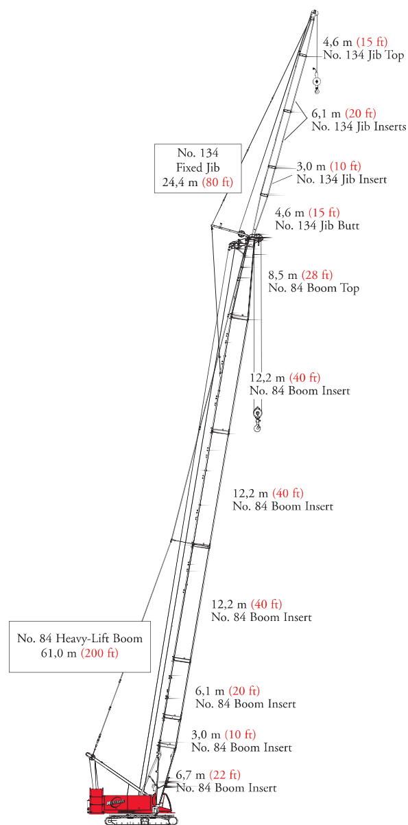
Model 555 No. 134 Fixed Jib on No. 84 Heavy-Lift Main Boom
