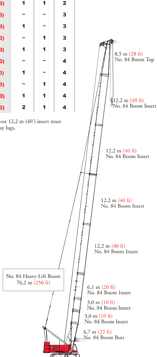
Model 555 No. 84 Heavy-Lift Main Boom
